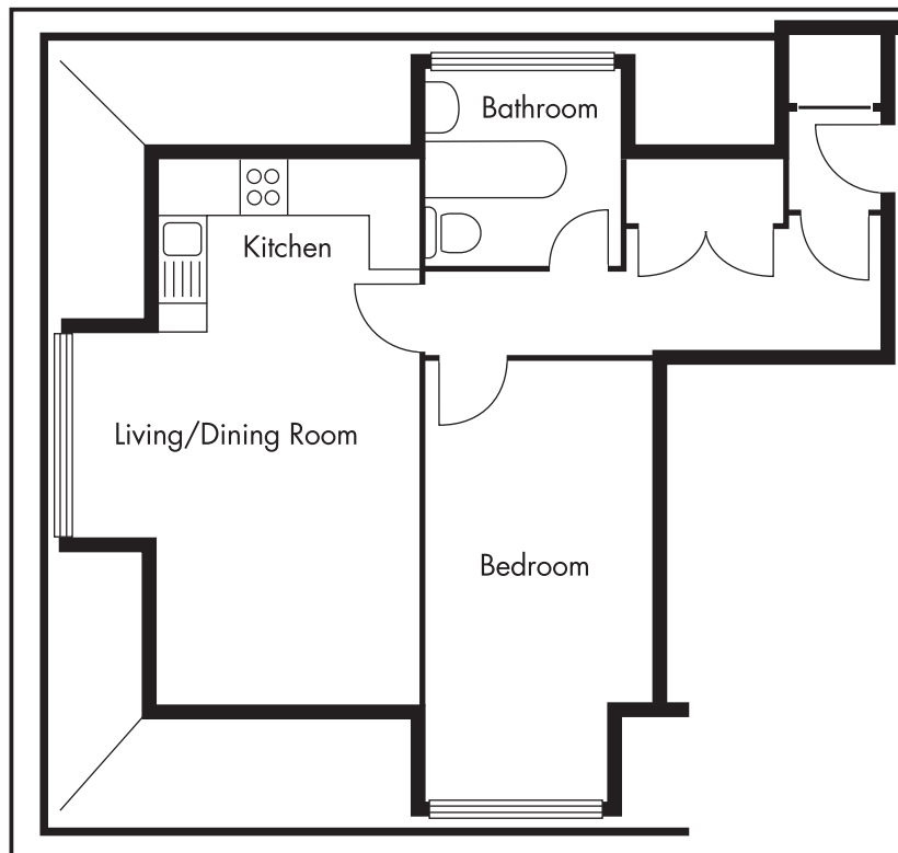
SECOND FLOOR
